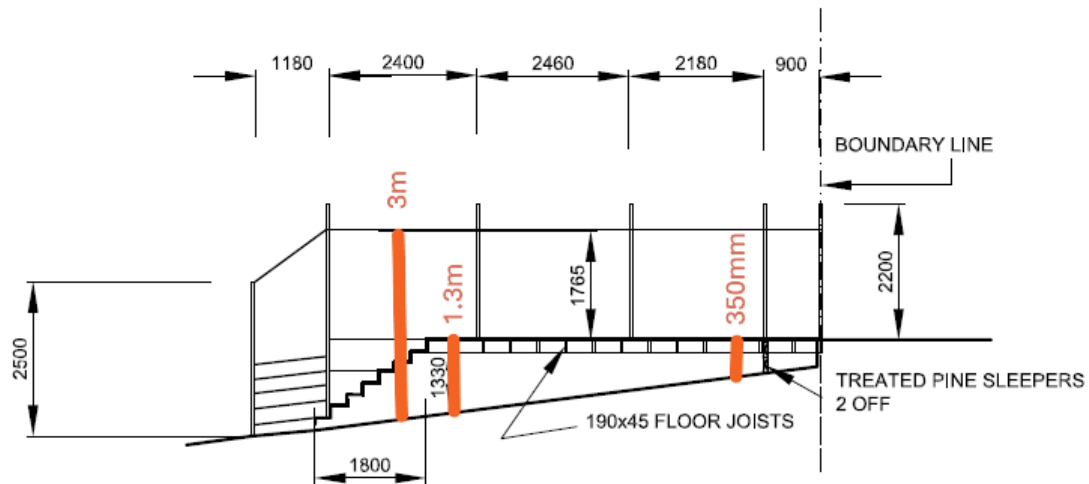
SIDE ELEVATION SECTION VIEWED FROM UNIT 2
