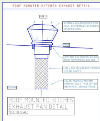
Vertical fan installation
